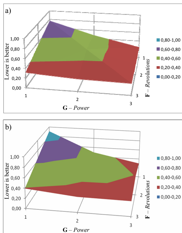
Fig. 6. Results of multi-criteria analysis a) variant 1; b) variant 2
