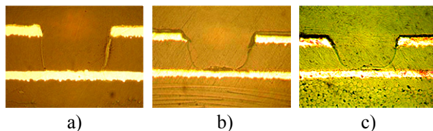
Fig. 5. The estimation of microvia bottom cleanness
