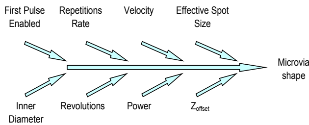
Fig. 1. Reason-result graph for process of blind microvia forming by spiral method
