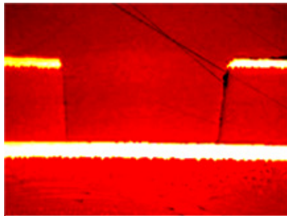
Fig. 7. Cross-section of 150 \mu\text{m} microvia formed in verifying experiment
