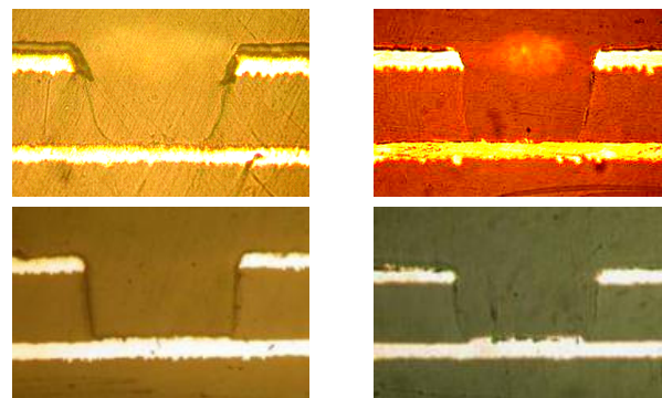
Fig. 2. Examples of cross-sections of 150 \mu\text{m} microvias formed in experiment
