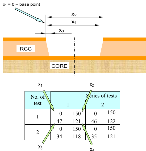
Fig. 3. Methodology of measurements of microvia dimensions
